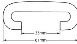
S-8133FWNX 81 Style TuffFlex Handrail Category: Handrails
