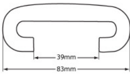
S-8339FWNX 83 Style TuffFlex Handrail Category: Handrails
