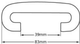
MI-8339FWCX 83 Style TuffFlex Handrail Category: Handrails
