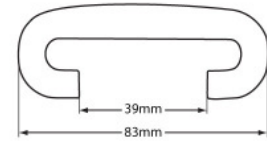
S-8339FWCX 83 Style TuffFlex Handrail Category: Handrails
