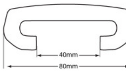
W-8040EFSCw 80 Style TuffFlex Handrail Category: Handrails
