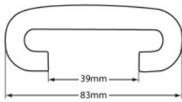
O-8339NTAABZ 83 Style NT Handrail Category: Handrails
