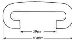
MI-8339FWVNX 83 Style TuffFlex Handrail Category: Handrails
