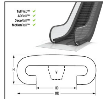
T-8942VWCX 89 Style TuffFlex Handrail Category: Handrails
