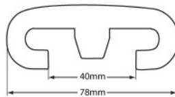
S-7840VWNX 78 Style TuffFlex Handrail Category: Handrails
