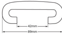
T-8942NTAABZ 89 Style NT Handrail Category: Handrails
