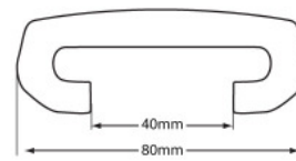
W-8040EFSM 80 Style TuffFlex Handrail Category: Handrails
