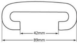
T-8942FWNX 89 Style TuffFlex Handrail Category: Handrails
