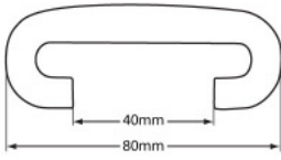
S-8040NTAABZ 80 Style NT Handrail Category: Handrails
