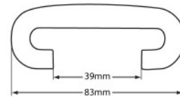
MI-8339NTAABZ 83 Style NT Handrail Category: Handrails
