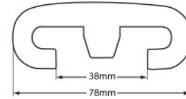
F-7838VWVNX 78 Style TuffFlex Handrail Category: Handrails
