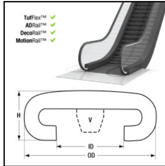
K-8942VWVNX 89 Style TuffFlex Handrail Category: Handrails
