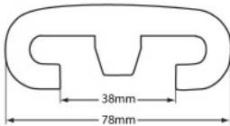
K-7838VWNX 78 Style TuffFlex Handrail Category: Handrails
