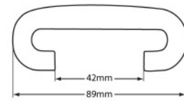
M-8942FWNX 89 Style TuffFlex Handrail Category: Handrails
