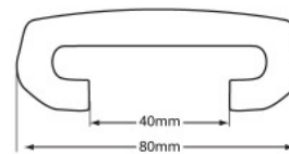
S-8040FWNX 80 Style TuffFlex Handrail Category: Handrails
