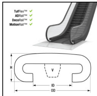
T-8942VWNX 89 Style TuffFlex Handrail Category: Handrails
