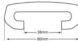
K-8038FWNX 80 Style TuffFlex Handrail Category: Handrails
