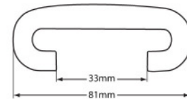
O-8133FWNX 81 Style TuffFlex Handrail Category: Handrails
