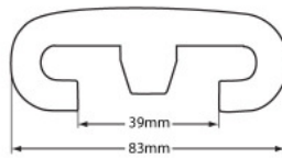
O-8339VWNX 83 Style TuffFlex Handrail Category: Handrails
